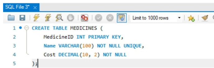
Figure 18: Creating the MEDICINES table.
